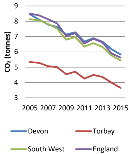
Figure 7 – CO 2 Emissions per Person, per Year
