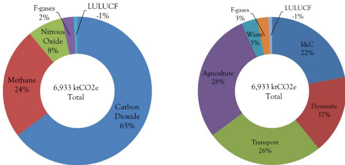
Figure 9 - Split of GHG emissions by gas and sector for Devon in 2015 (note: carbon dioxide emissions from agriculture are allocated to the I&C sector, and F-gas %s differ due to rounding)
