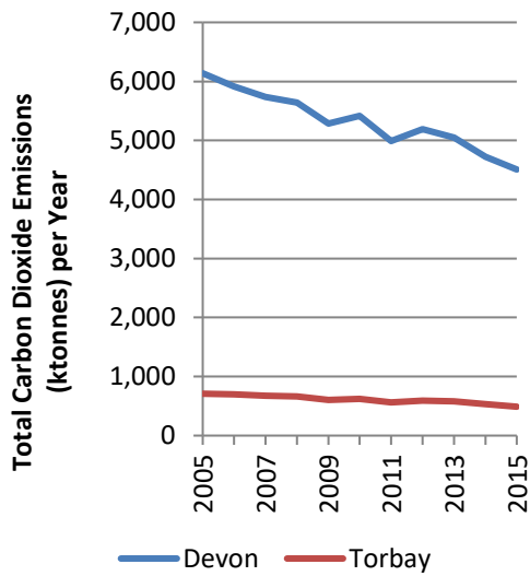
Figure 6 – CO 2 Emissions per Year
