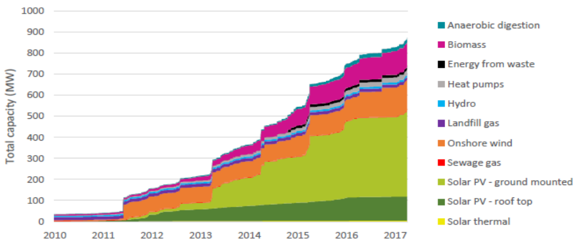
Figure 4 – Increase in renewable energy capacity in Devon since 2010
