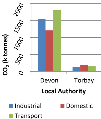
Figure 8 - Carbon Dioxide Emissions by source in 2015
